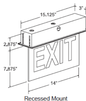
Recessed Mount
