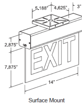
Surface Mount
